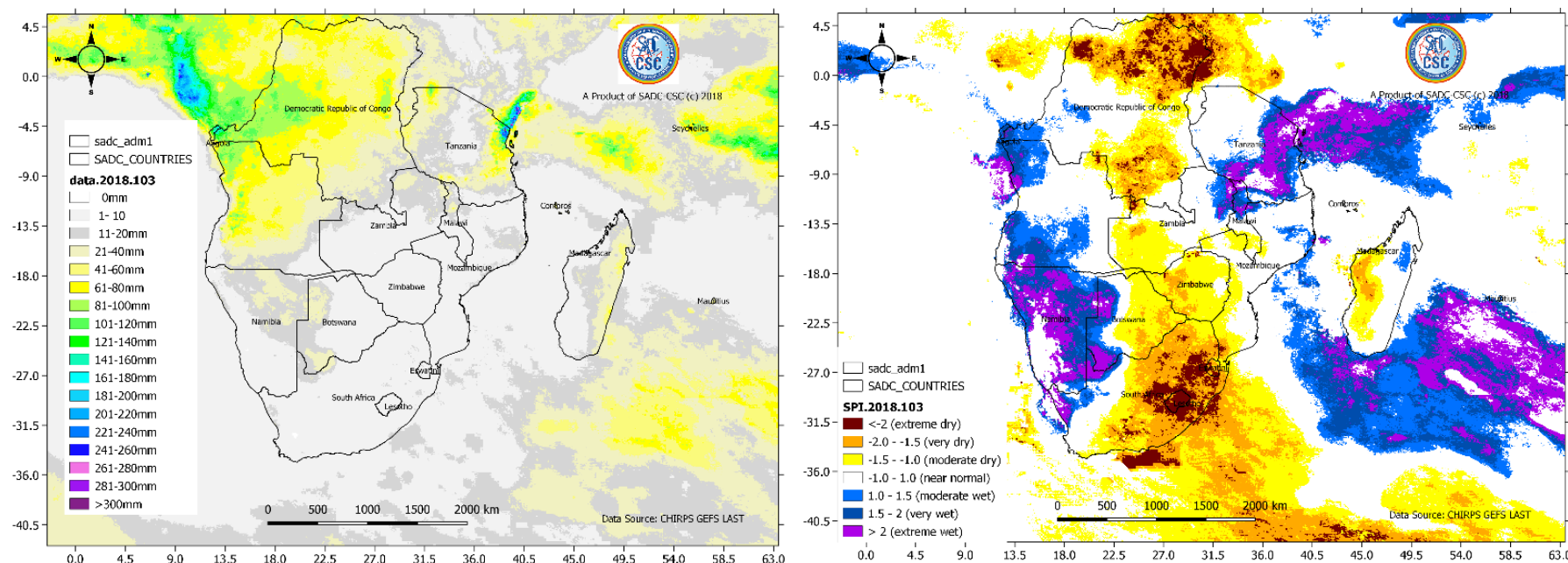
Figure 1: Total rainfall during the third dekad (21-30) (left) and SPI (right) for the third dekad of October 2018
