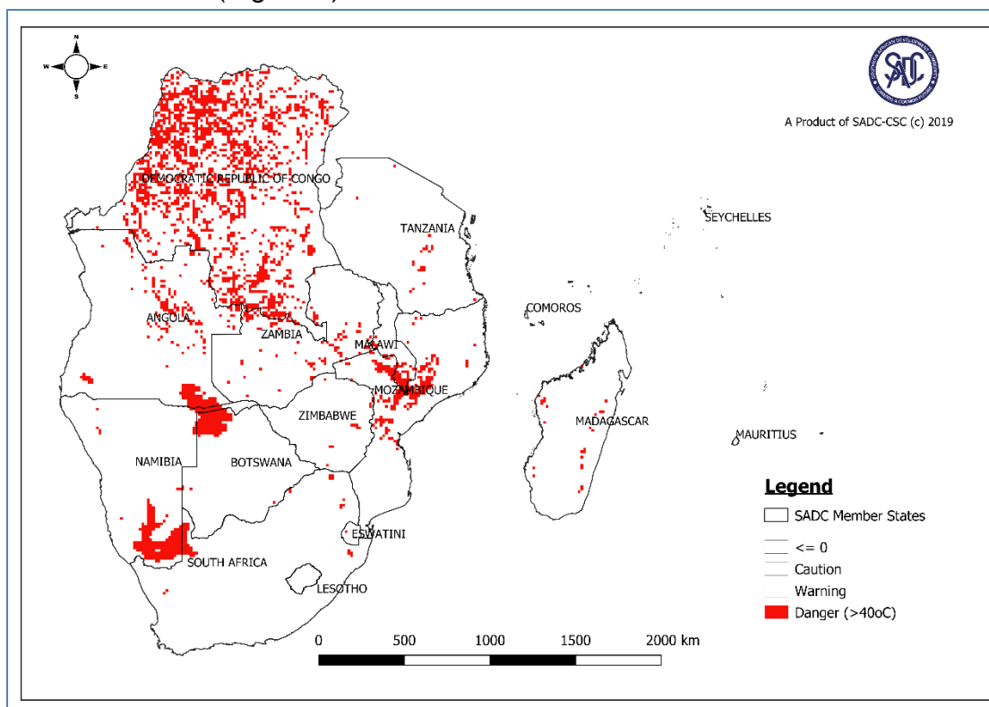
Figure 2: Extreme high temperature forecasted for 20 – 26 November 2019 (Source: SADC-CSC-WRF Model )
