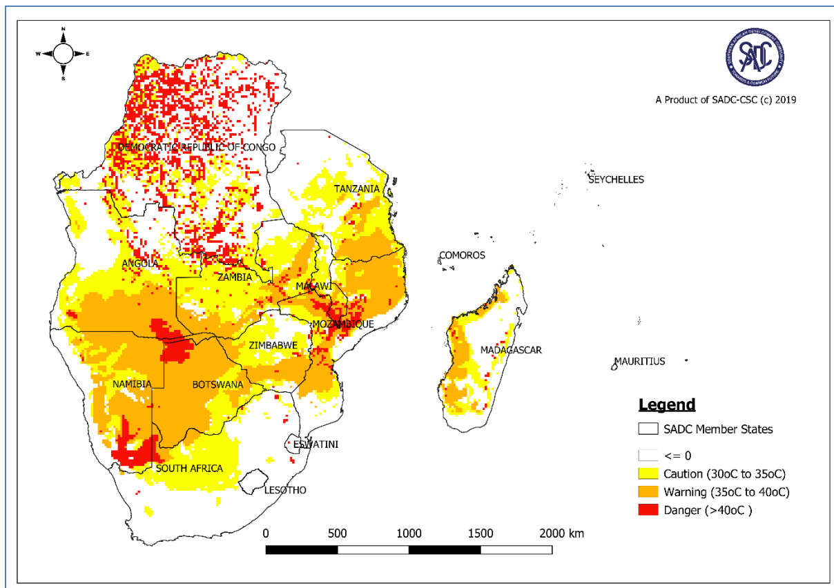
Figure 1: High temperature forecast for the period 20– 26 November 2019 (Source: SADC-CSC-WRF Model )
