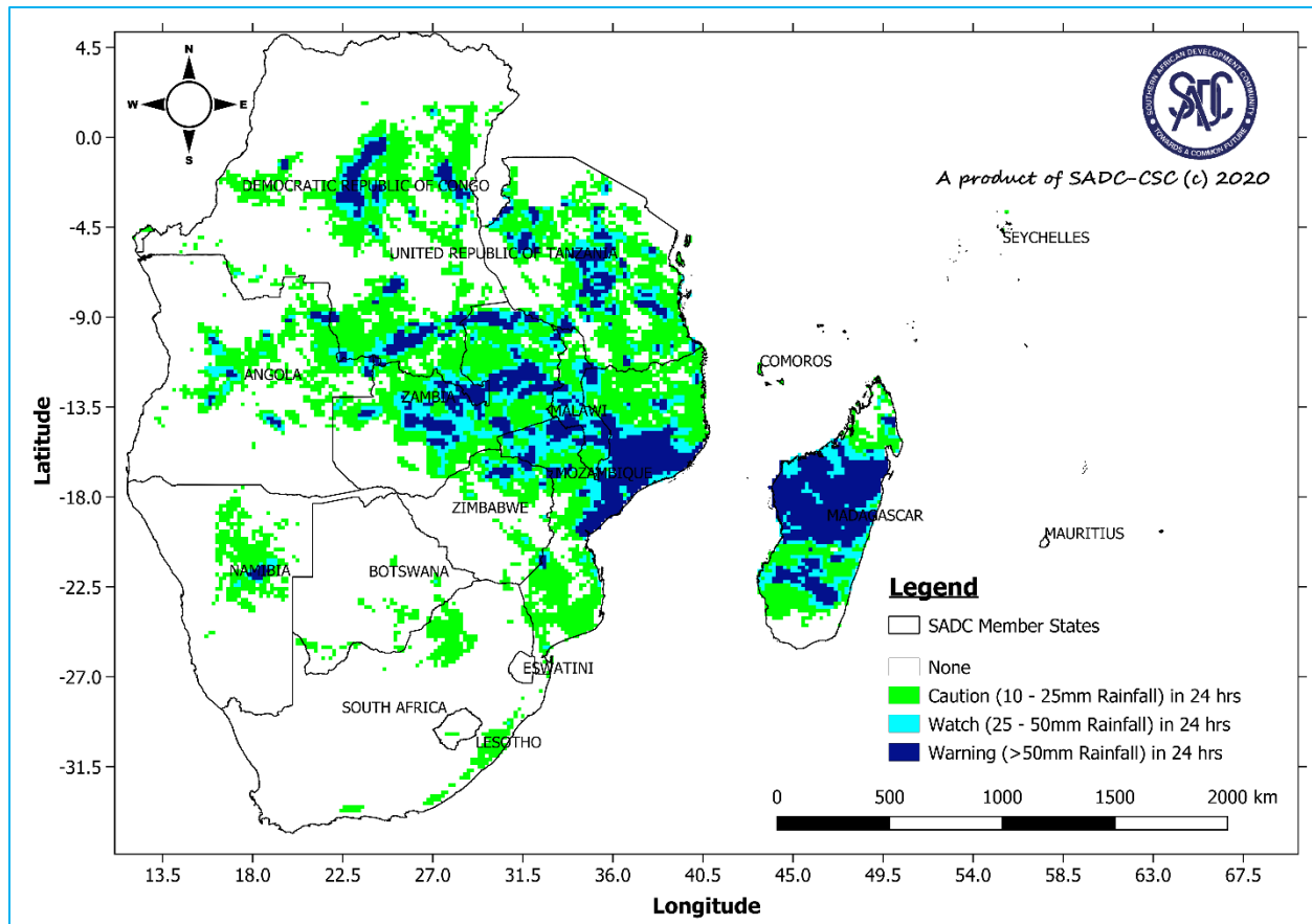
Figure 1: SADC Region's heavy rainfall advisory for the period 15 to 22 January 2020 (Source: SADC-CSC-WRF GFS Model)
