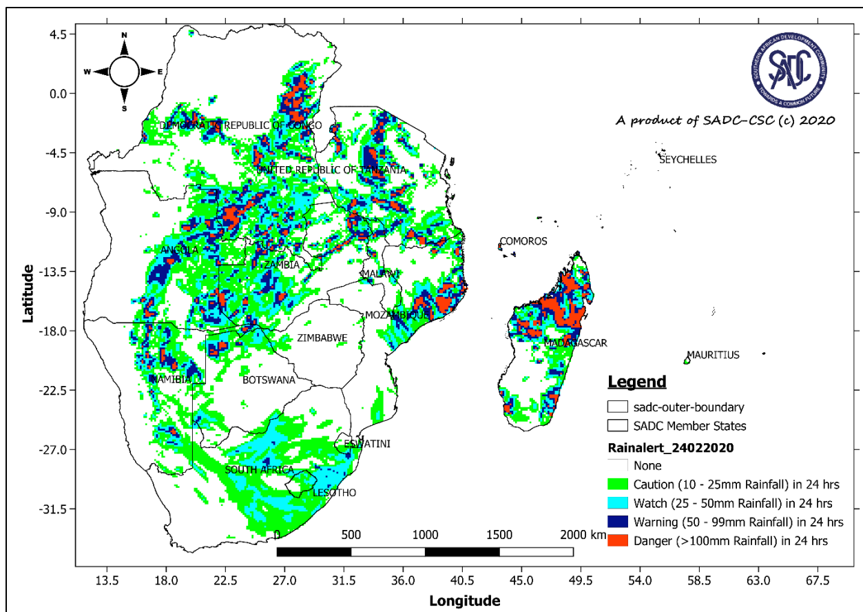
Figure 1: SADC Region's heavy rainfall advisory for the period 24 February to 01 March 2020 (Source: SADC-CSC-WRF GFS Model)
