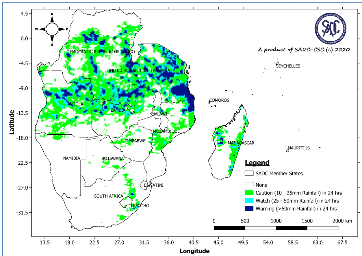
Figure 1: SADC Region's heavy rainfall advisory for the period 31 January to 06 February 2020 (Source: SADC-CSC-WRF GFS Model)
